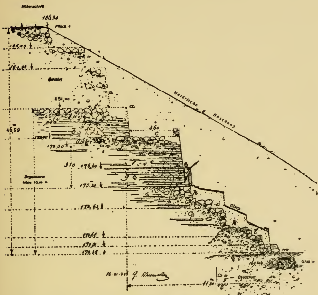
FIG. 2.—Section of the Town Wall of Megiddo. (By Schumacher.)
